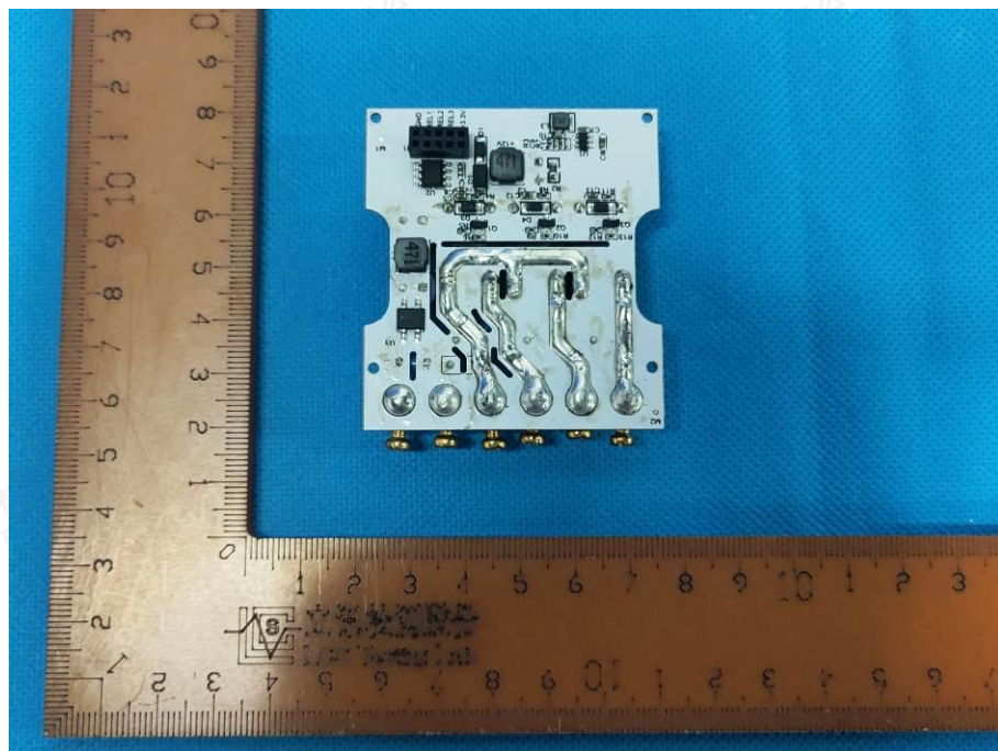
Figure 10 PCB view (for model LT-03)
