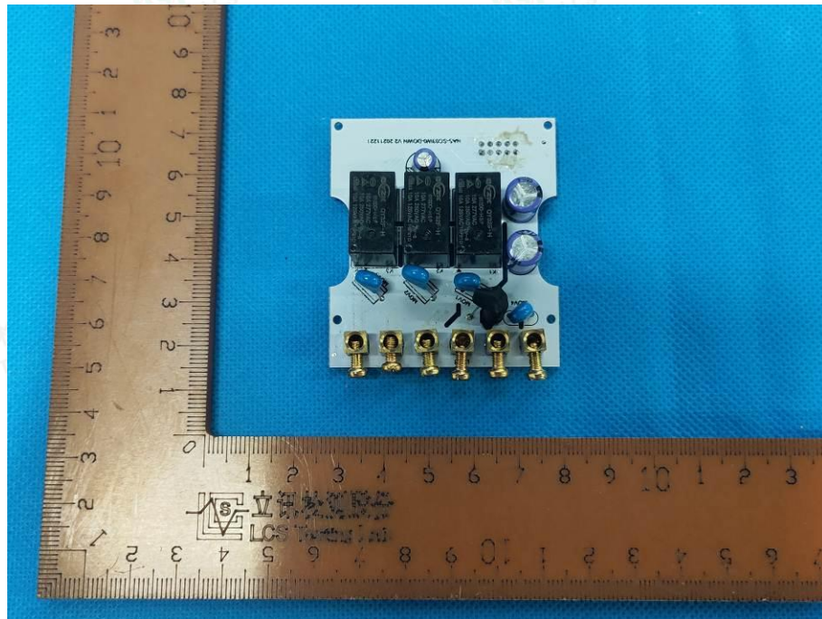
Figure 9 PCB view (for model LT-03)
