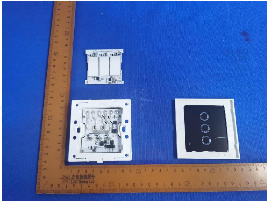
Figure 5 Internal view (for model LT-03)
