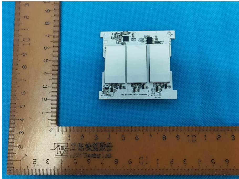
Figure 6 PCB view (for model LT-03)
