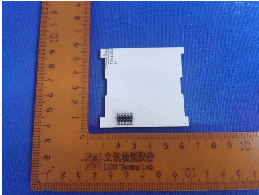
Figure 7 PCB view (for model LT-03)
