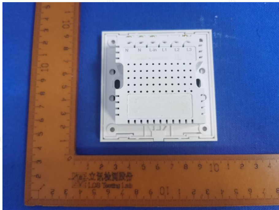
Figure 2 External view (for model LT-03)
